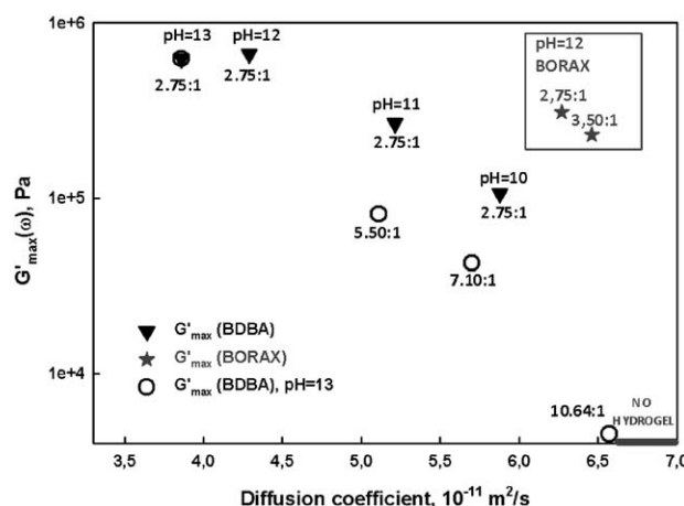
FIGURE 6 G'_{\text{max}}(\omega) values of hydrogels versus diffusion coefficients of solutions containing polymers treated with a cross-linker at various pHs and a diol to boronic acid site molar ratio of 2.75:1.
